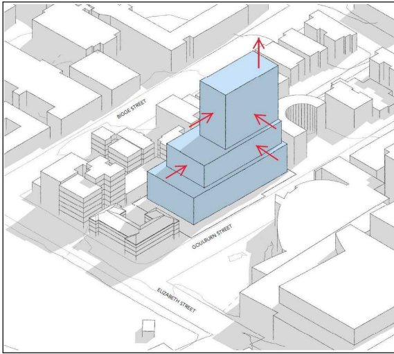
Setbacks at various level were maximised to introduce a multilevel landscape. The envelope is made more tall end slender to reduce the width of the shadow cast.
