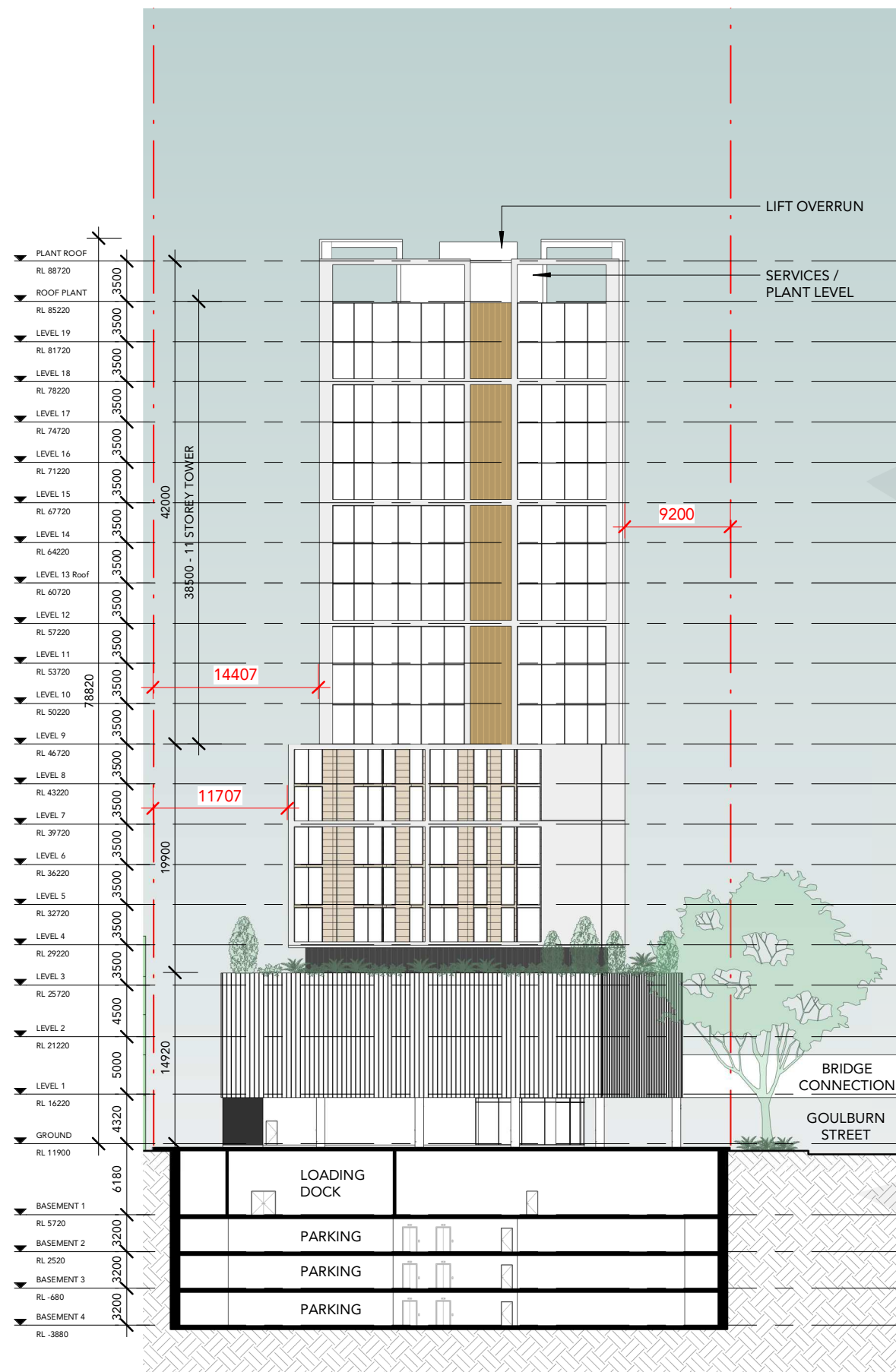
SOUTH ELEVATION
