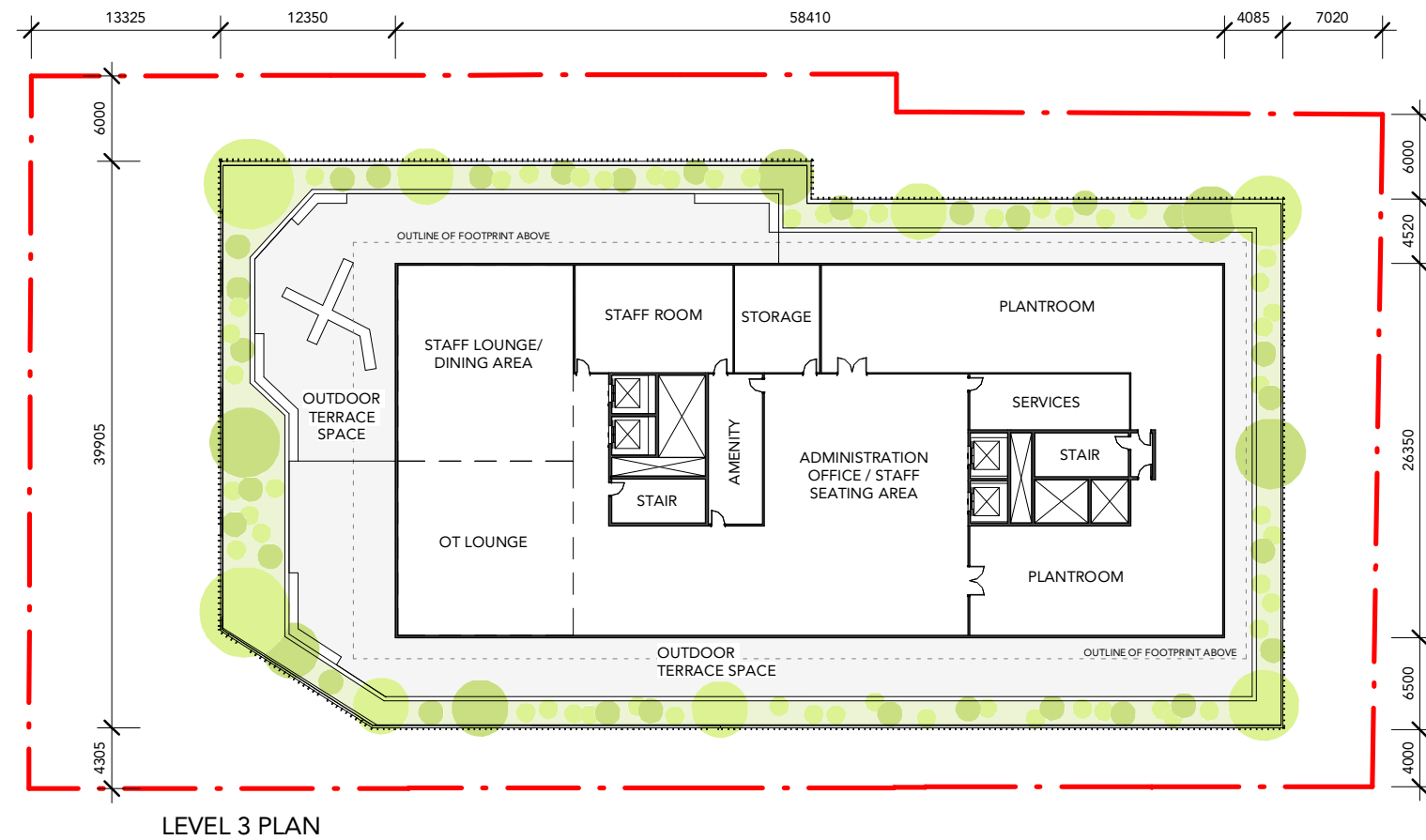
LEVEL 3 PLAN
